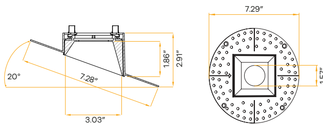
Square Flangeless
