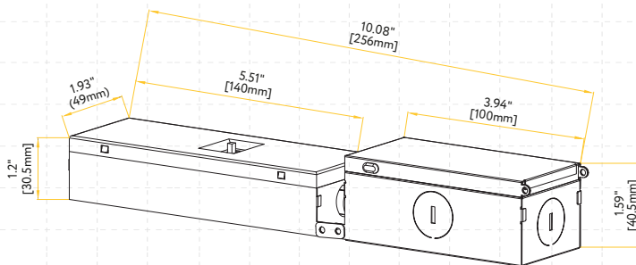
Bendable Driver Box for G-23500 & G-23505
