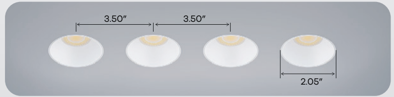
Double Kit
