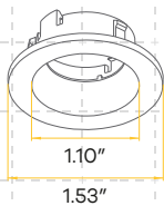
Round Trimmed
