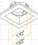
Square Trimmed
